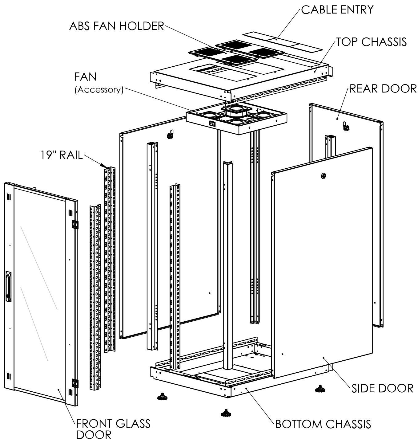
Exploded view
