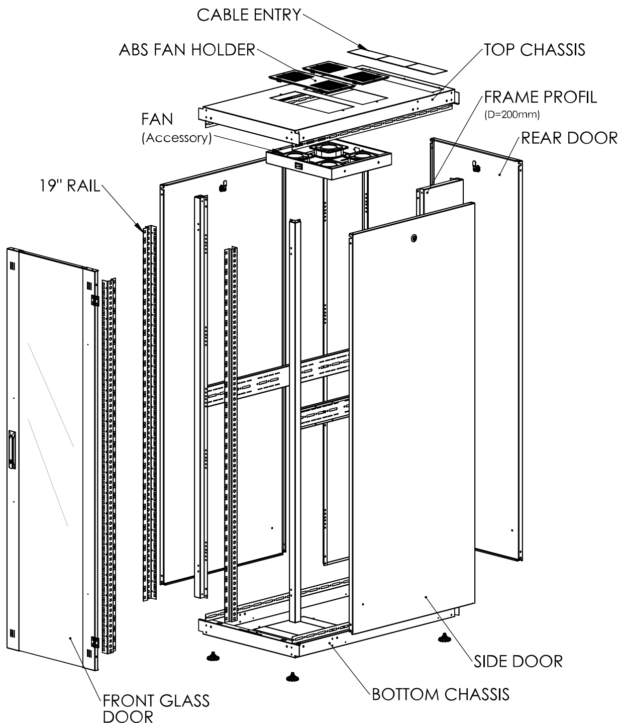
Exploded view
