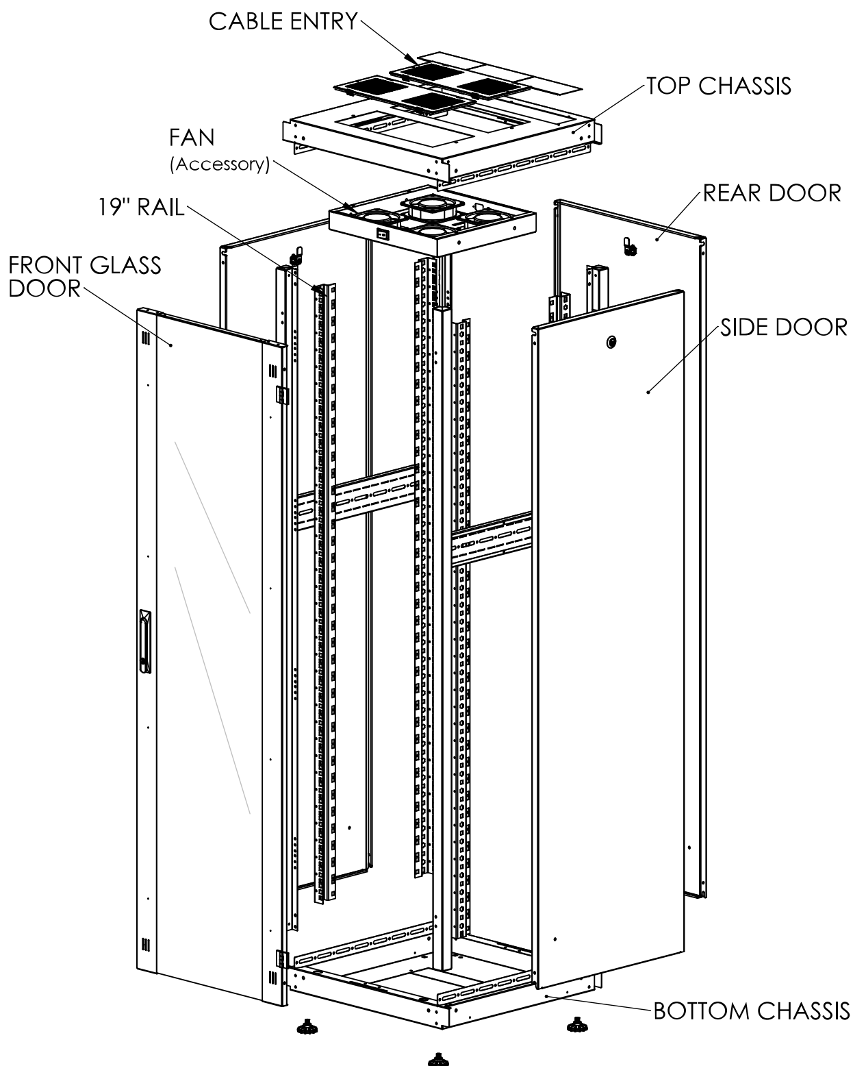
Exploded view
