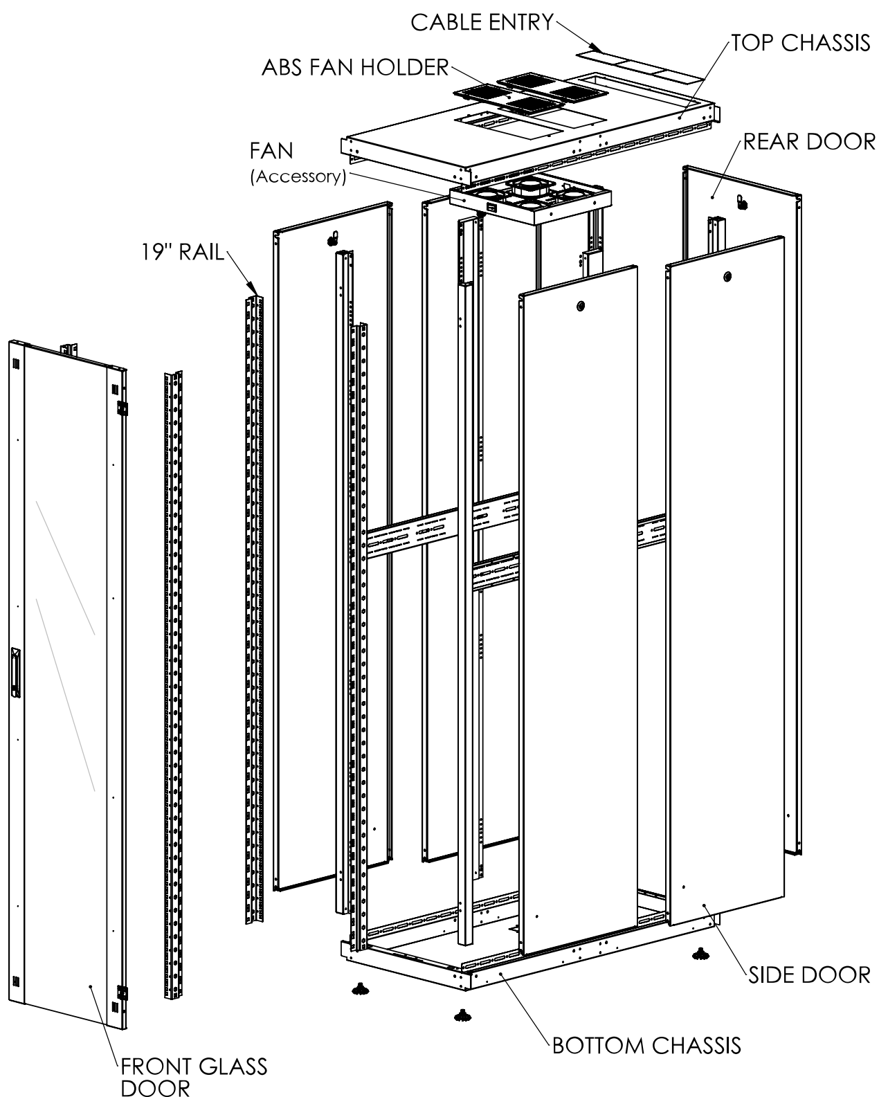
Exploded view
