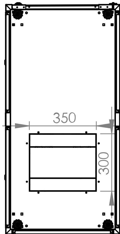
Bottom view
