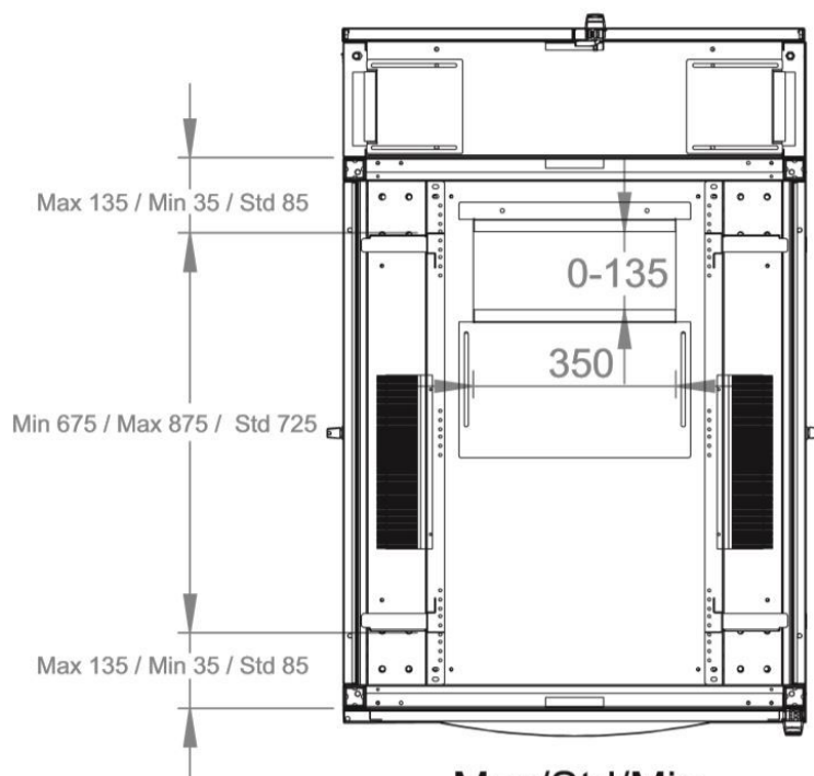
Max/Std/Min Equipment mounting Distance
