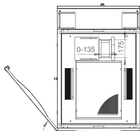
0°-230° Front door opening angle
