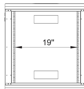
Front inside view
