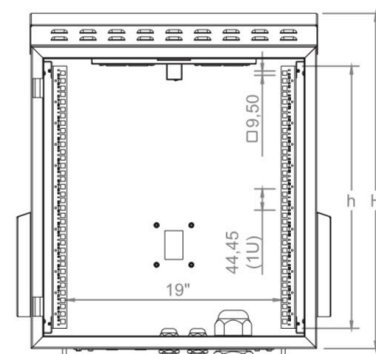
Inside view
